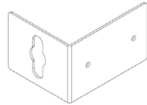
251-01-0104-00 Dimensions (WxDxH): 95mm x 75mm x 60mm L Bracket with rounded and extended length U-shaped holes to mount a single PDU.
