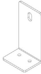
251-01-0102-00 Dimensions (WxDxH): 93mm x 40mm x 50mm L Bracket with rounded and small-sized U-shaped holes to extend the height of a PDU.
