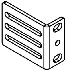
251-02-0011-00 Dimensions (WxDxH): 53.2mm x 43.6mm x 21.3mm L Bracket with rounded, small-sized U-shaped and extended length U-shaped holes to extend the height of a PDU.
